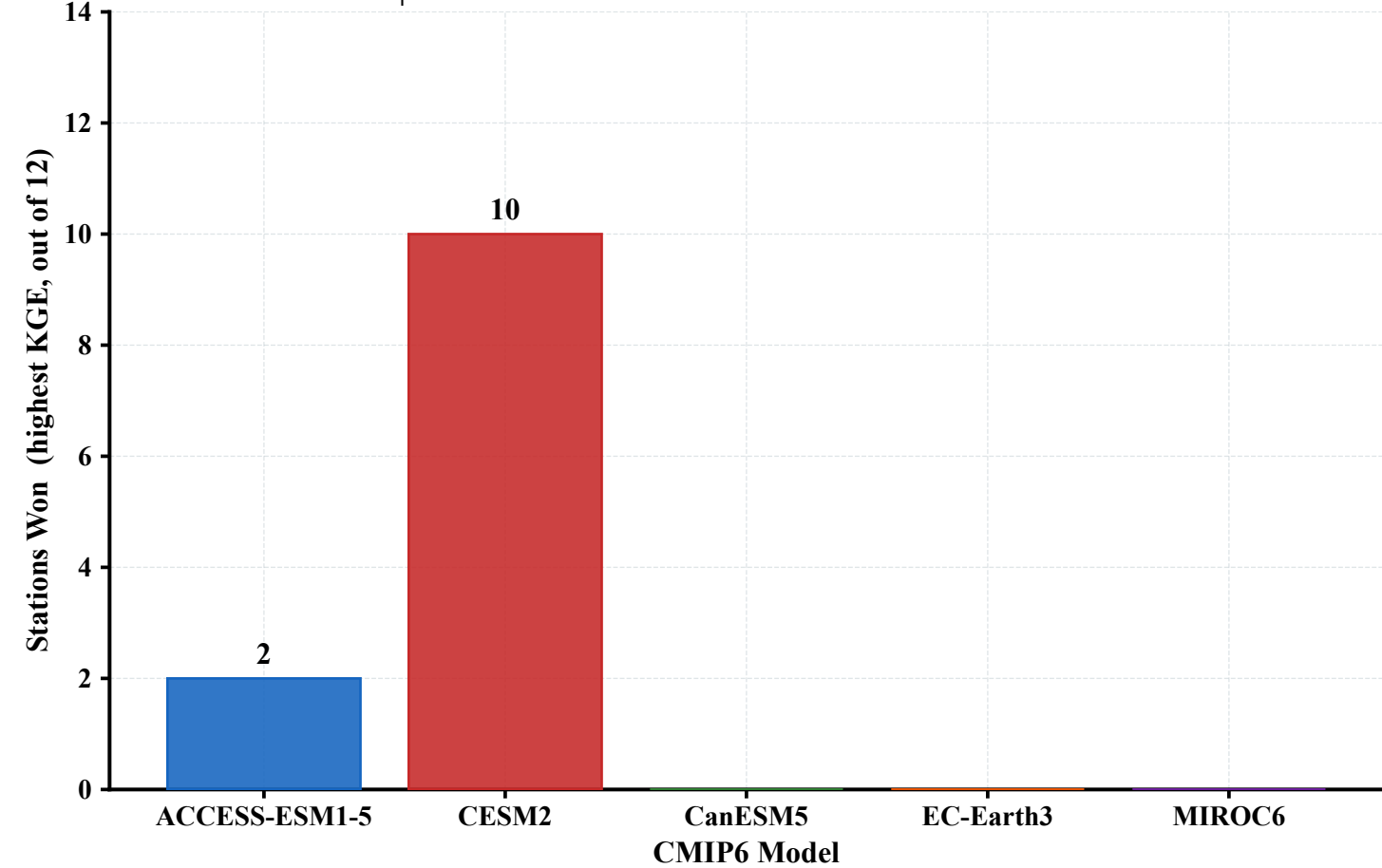
(d) Best Model per Station — After Bias Correction Total = 12 stations | Metric = KGE
