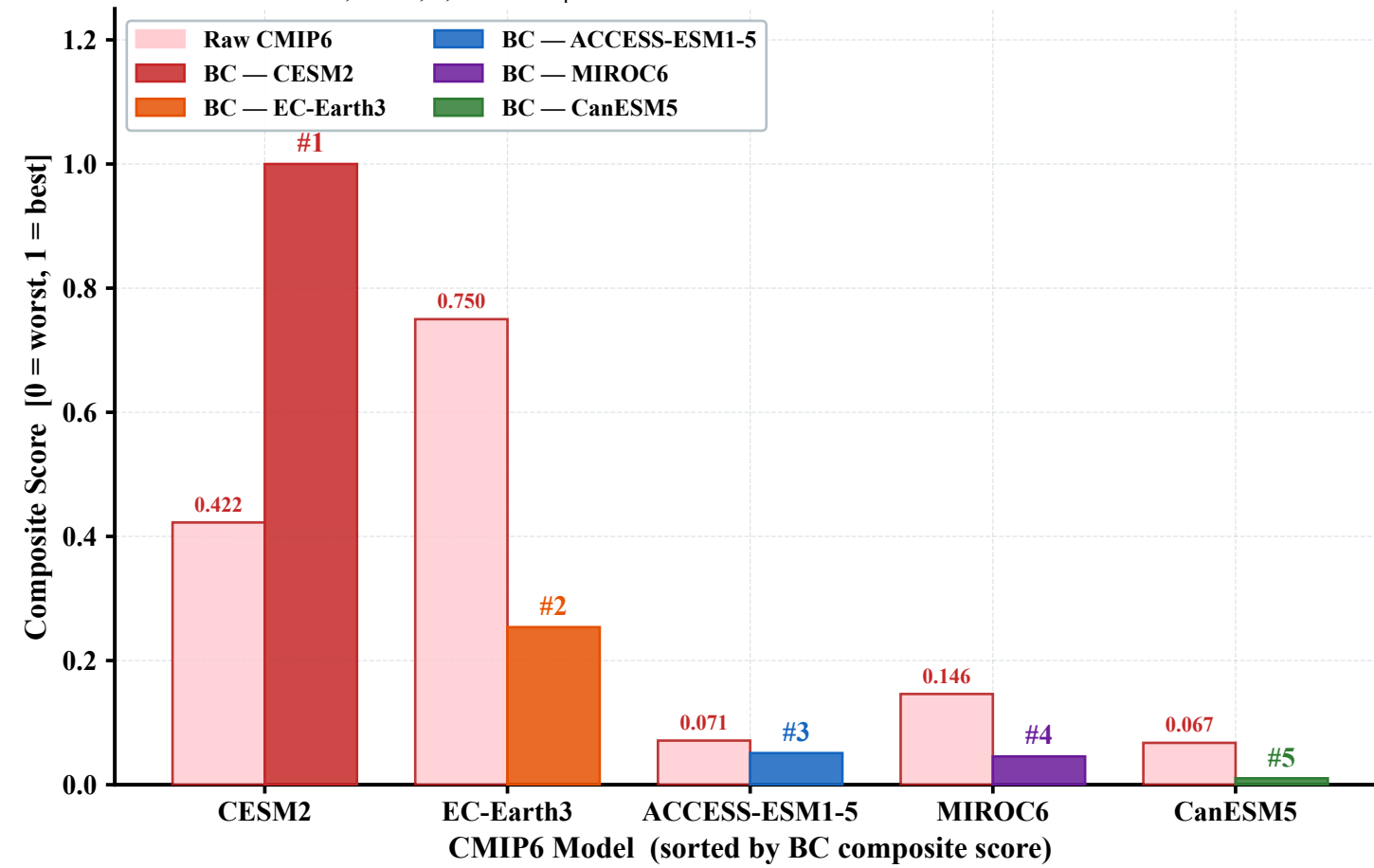
(a) Composite Performance Score — Raw vs Bias-Corrected Based on KGE, NSE, r, RMSE | Numbers = BC rank
