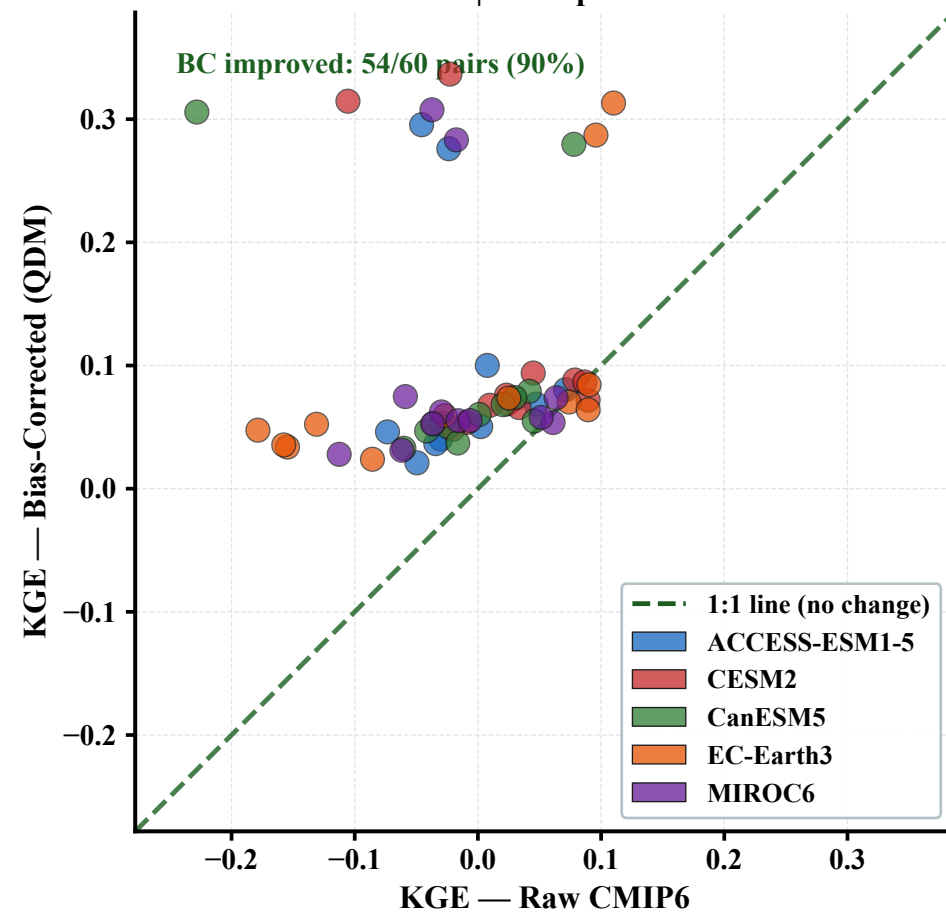
(c) Station-Level KGE: Raw vs Bias-Corrected All models combined | Each point = 1 model × 1 station
