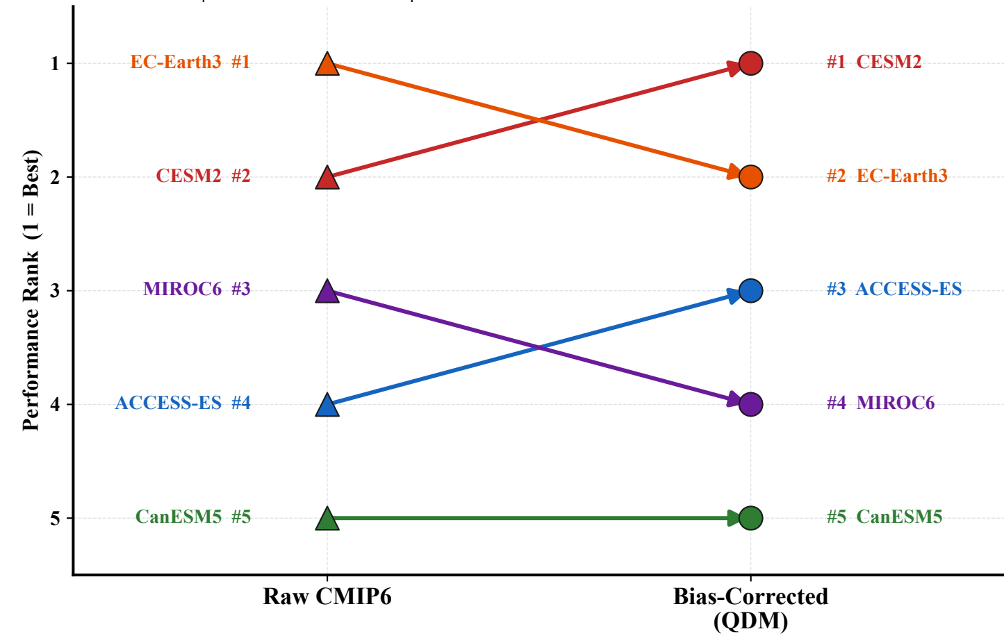
(b) Model Ranking Change After QDM Bias Correction ▲ = Raw | ● = Bias-Corrected | Arrow = rank shift
